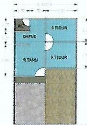
DENAH 6X10
